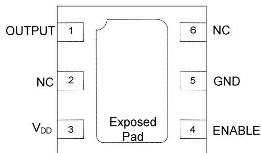
U-DFN2020-6
