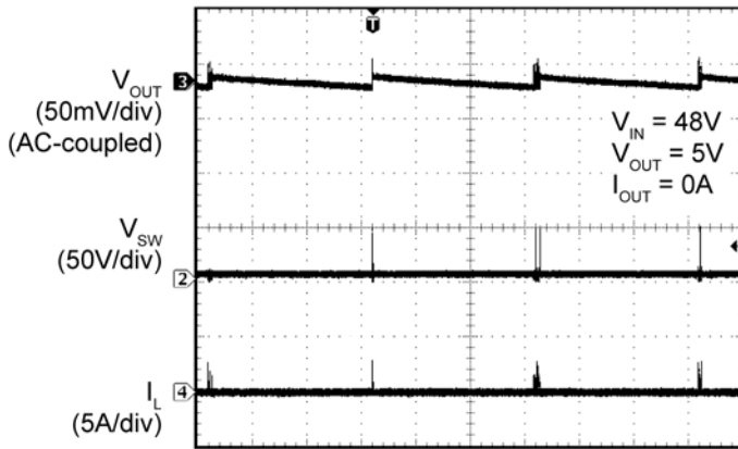
MIC2103 Switching Waveforms I_{OUT} = 0A (DCM)
