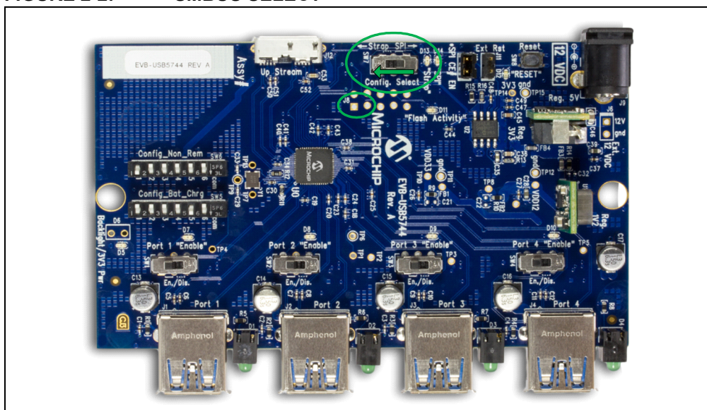
FIGURE 2-2: SMBUS SELECT
