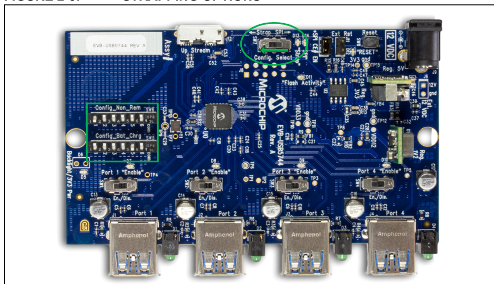
FIGURE 2-3: STRAPPING OPTIONS
