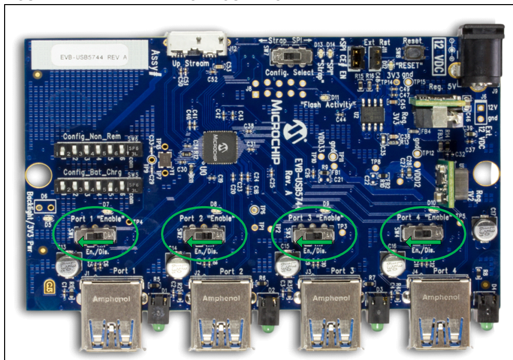
FIGURE 2-4: INITIAL CONFIGURATION
