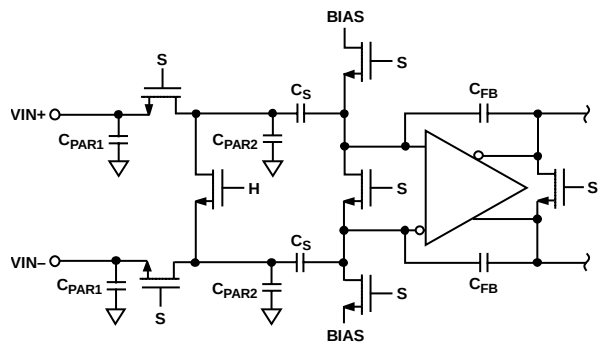
Figure 48. Switched-Capacitor Input
