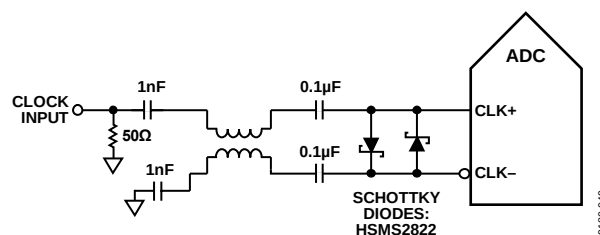
Figure 55. Balun-Coupled Differential Clock (Up to 640 MHz)
