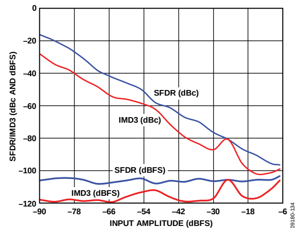
Figure 34. AD9644-155 Two-Tone SFDR/IMD3 vs. Input Amplitude ( A_{IN} ) with f_{IN1} = 169.1 MHz, f_{IN2} = 172.1 MHz, f_s = 80 MSPS
