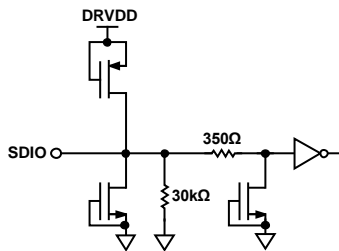
Figure 44. Equivalent SDIO Circuit
