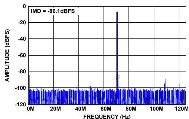
FIGURE 20. TWO-TONE SPECTRUM AT 70MHz
