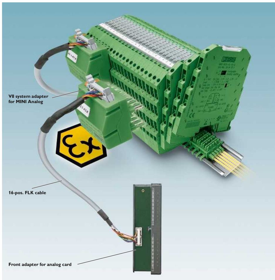
System cabling with a front adapter
