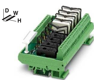
8-channel for relays with a PDT contact
