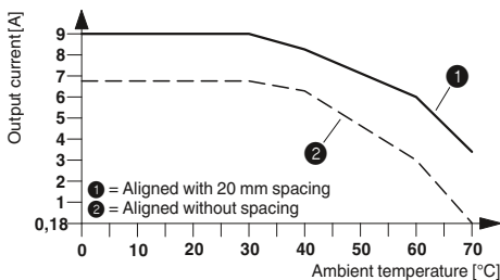
Derating curve for ELR H5-SC-24DC/500AC-9 100% operating time
