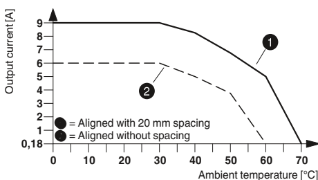
Derating curve for ELR H5-SC-230AC/500AC-9 100% operating time
