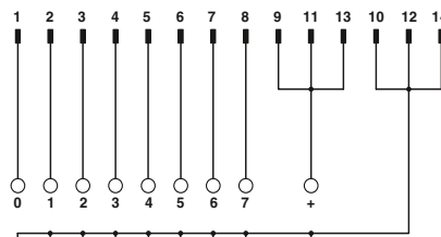
Connection scheme VIP-2/.../FLK14/8M/PLC
