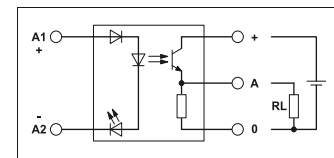
Figure 4: 3-conductor output
