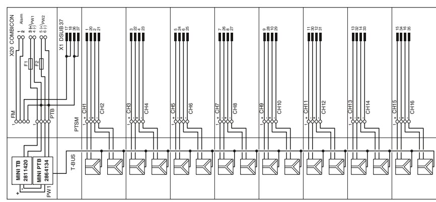
TC-D37SUB-ADIO16-M-P-UNI and TC-D37SUB-AIO16-M-PS-UNI connection scheme
