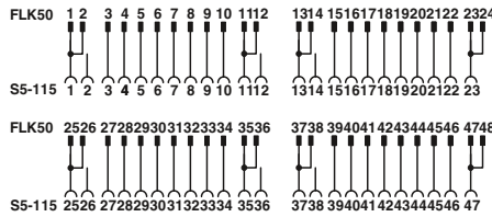
Connection scheme: FLKM S115/S7/FLK50/PLC/SO137
