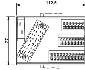
Dimensional drawing for UMK-EC 56/25/EX/Front 2,5 V/L
