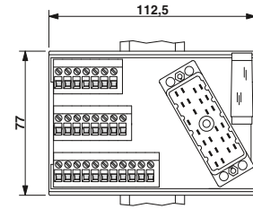
Dimensional drawing for UMK-EC 56/25/EX/Front 2,5 V/R
