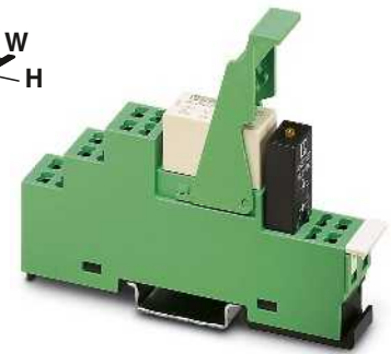
PR1 relay module with 1 PDT relay
