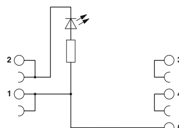
PLC-VT/ACT/LA connection scheme
