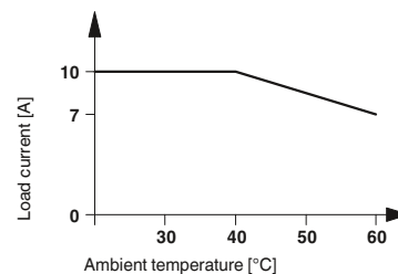
Derating curve for PLC-...24DC/24DC/10/R
