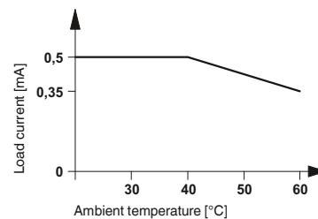
Derating curve for PLC-...24DC/48DC/500/W
