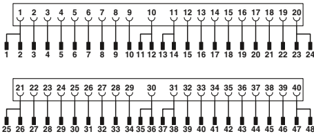
Connection scheme FLKM 50-PA-S300/SO167
