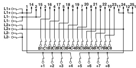
FLKM-D25 SUB/B/KDS3-MT/TU810/P connection scheme
