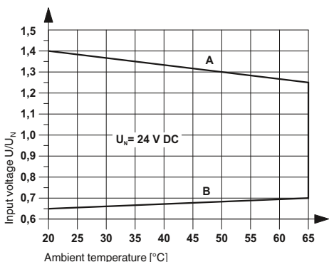
Curve A Maximum continuous voltage at limiting continuous current = 3 A
