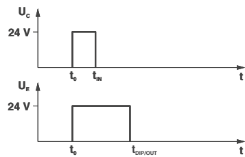
Input pulse t_1 < \text{set output pulse } t_3 (no restart when triggered again)
