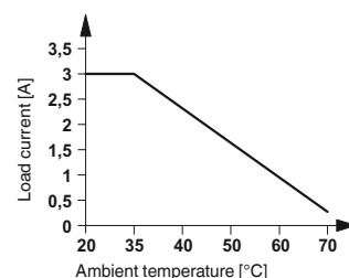
Derating curve for PLC-OSP...110DC/3RW
