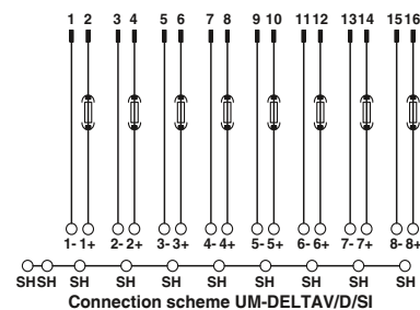
Connection scheme UM-DELTA V/D/SI
