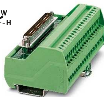
37-pos. with screw or push-in connection
