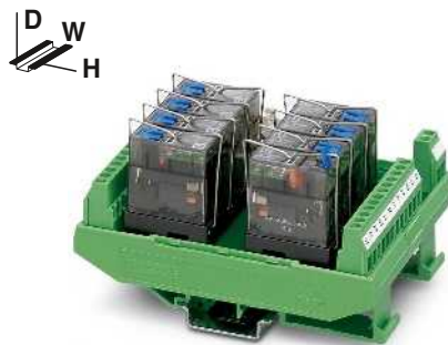
Output module with 8 miniature relays, 1 PDT with detectable manual operation
