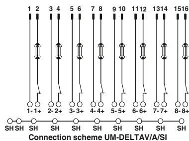
Connection scheme UM-DELTA V/A/SI
