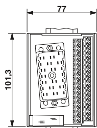
Dimensional drawing for UMK-EC90/32/EX-XOL
