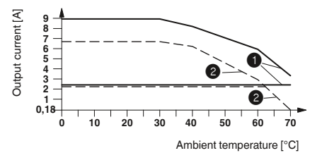
Derating curve ELR H3-IES-SC-24DC/500AC-2 and ELR H3-IES-SC-230AC/500AC-9 100% operating time
