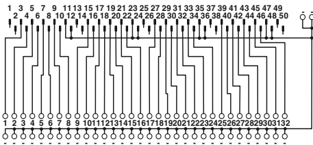
FLKM 50/32M/DV connection scheme
