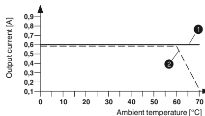
Derating curve ELR H3-I-SC-24DC/500AC-5 100% operating time
