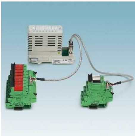
FLKM-D25 SUB/B/KDS3-MT/TU810 connection scheme
