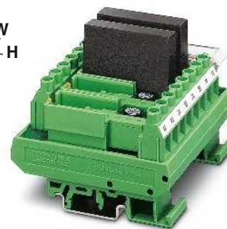
With light indicator and fuse, control logic positive switching
