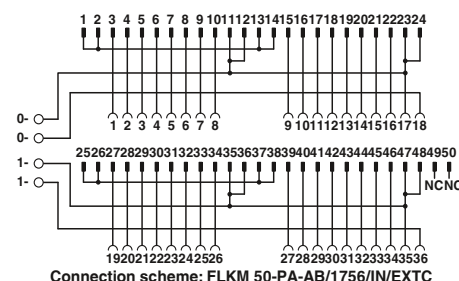
Connection scheme: FLKM 50-PA-AB/1756/IN/EXTC
