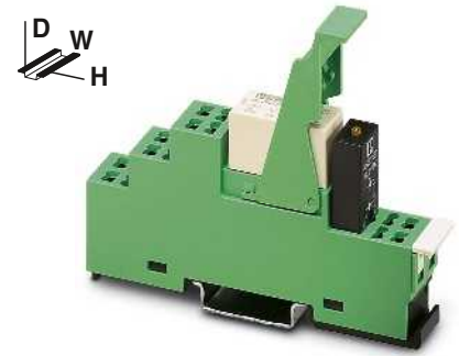
PR1 relay module with 1 PDT relay
