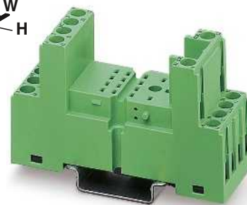
2/2-level design with screw connection
