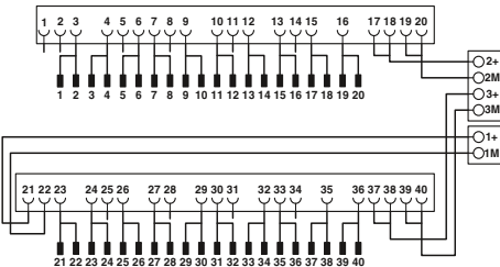
Connection scheme FLKM 50-PA/DO326/S7-300
