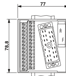
Dimensional drawing for UMK-EC56/25/EX-R
