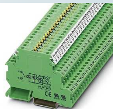
Relay module with manual switch and integrated relay
