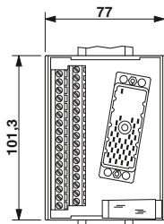
Dimensional drawing for UMK-EC56/32-XOR
