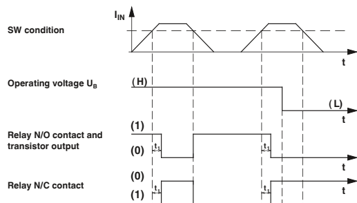
3) Quiescent current-controlled when threshold value is exceeded
