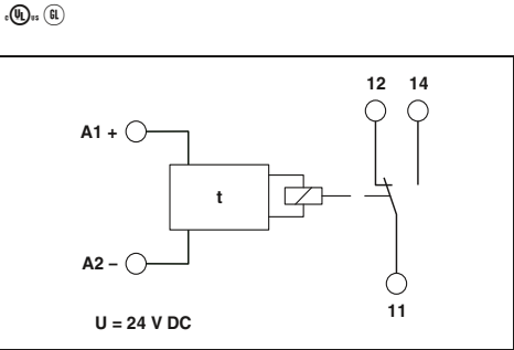
Timer relay with switch-on delay, voltage controlled
