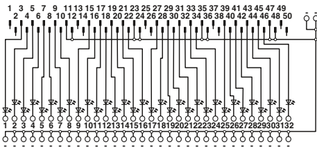
FLKM 50/32M/IN/LA/DV connection scheme
