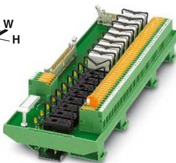
Output module for 16 miniature relays with knife/disconnect terminal blocks, 1 PDT
