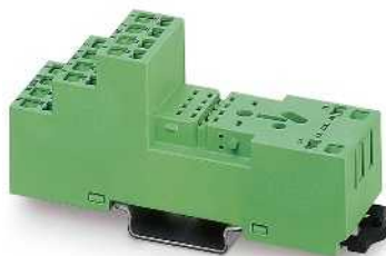
1/3-level design with spring-cage connection
