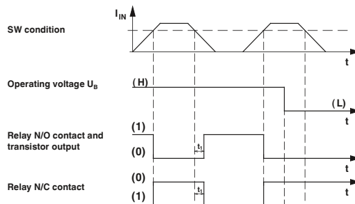
2) Operating current-controlled when below the threshold value
