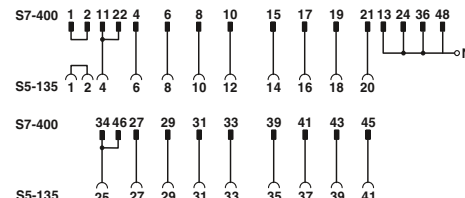
Connection scheme: FLKM S135/S400/SO124
