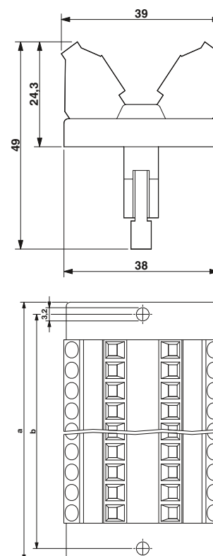
Dimensional drawing DFLK:
