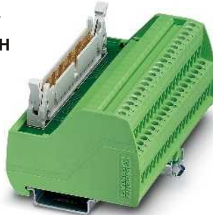
Passive interface modules for input/output with screw connection
