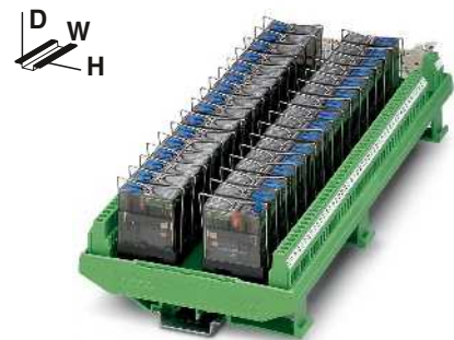
Output module with 32 miniature relays, 1 PDT with detectable manual operation
