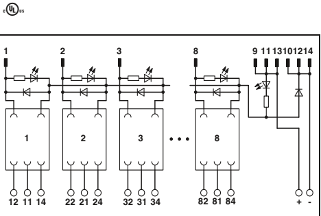
Output module with eight miniature relays, 1 PDT
