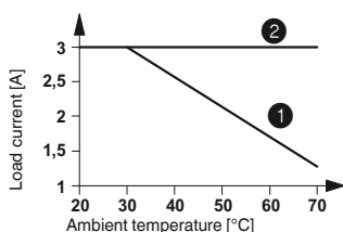
Derating curve for PLC-OSP...24DC/3RW
