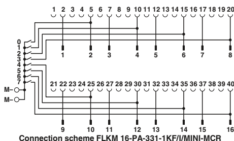
Connection scheme FLKM 16-PA-331-1KF/I/MINI-MCR
