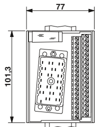
Dimensional drawing for UMK-EC90/32/EX-XUL
