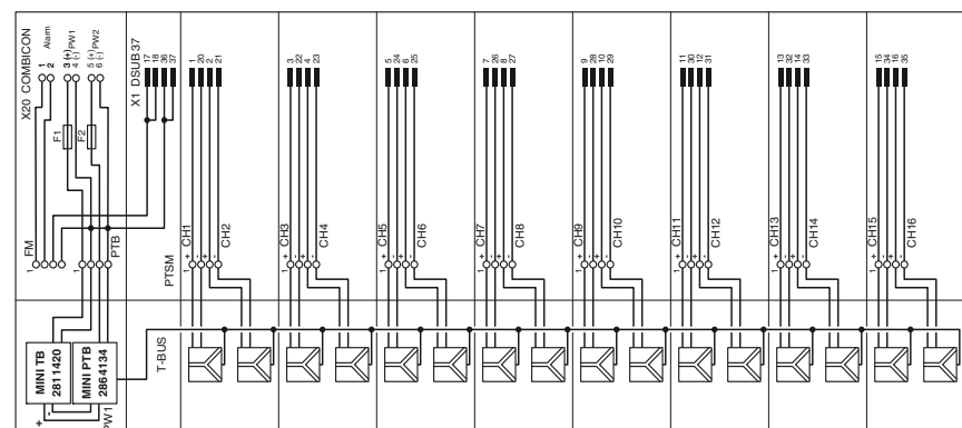
TC-D37SUB-ADIO16-M-P-UNI and TC-D37SUB-AIO16-M-PS-UNI connection scheme
