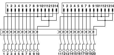
FLKM-2FLK14/KDS3-MT/PPA/S7 connection scheme
