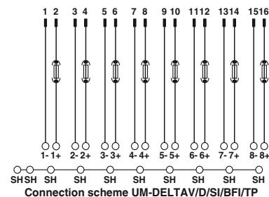
Connection scheme UM-DELTA V/D/SI/BFI/TP
