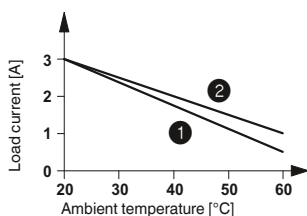
Derating curve for ST-OV 3-24DC/400AC/3
