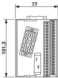
Dimensional drawing for UMK-EC38/38-XOL
