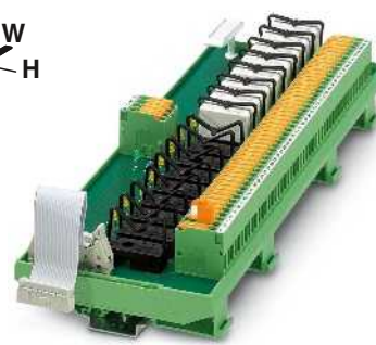
Output extension module for 16 miniature relays with knife/disconnect terminal blocks, 1 PDT
