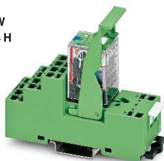
PR2 relay module with spring-cage connection
