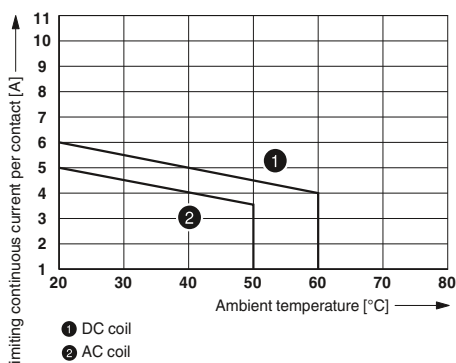
Contact derating
