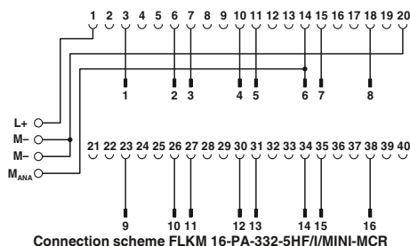
Connection scheme FLKM 16-PA-332-5HF/I/MINI-MCR
