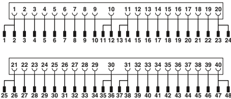
Connection scheme FLKM 50-PA-S300/SO167
