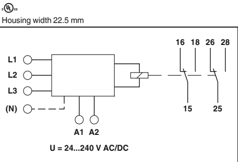
Undervoltage and phase monitoring, 400 V or 230 V
