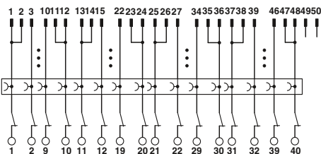
FLKM 50/KDS3-MT/PPA/S7-300 connection scheme
