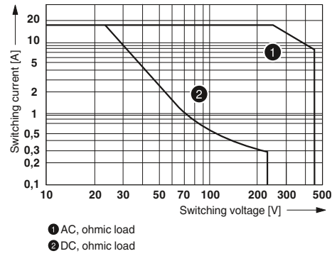
Interrupting rating
