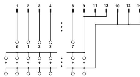
UM 45-FLK14/8IM/ZFKDS/PLC connection scheme
