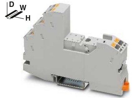
2 PDT relay base for miniature power relay
