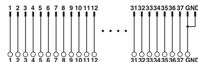
Connection scheme VIP-2/SC/D37SUB/M
