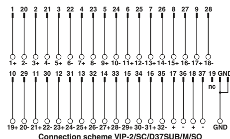
Connection scheme VIP-2/SC/D37SUB/M/SO
