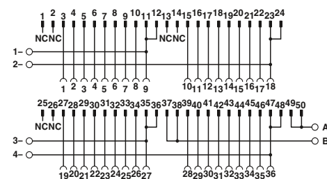
Connection scheme for FLKM 50-PA-GE/TKFC/RXI/IN
