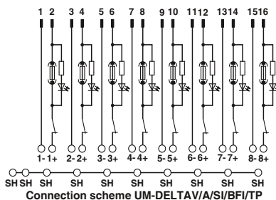
Connection scheme UM-DELTA V/A/SI/BFI/TP
