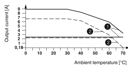
Derating curve ELR H5-IES-SC-24DC/500AC-2 and ELR H5-IES-SC-230AC/500AC-9 100% operating time
