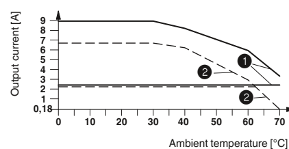
Derating curve ELR H3-IES-SC-24DC/500AC-2 and ELR H3-IES-SC-230AC/500AC-9 100% operating time
