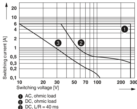
Electrical interrupting rating for PLC...21HC for high continuous currents
