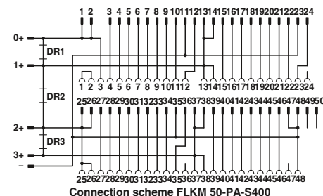
Connection scheme FLKM 50-PA-S400
