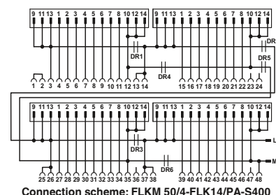
Connection scheme: FLKM 50/4-FLK14/PA-S400
