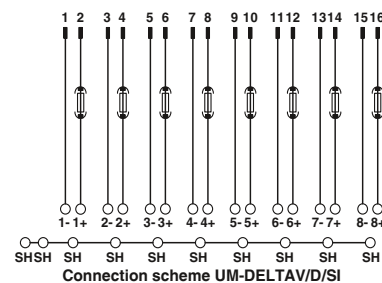
Connection scheme UM-DELTA V/D/SI
