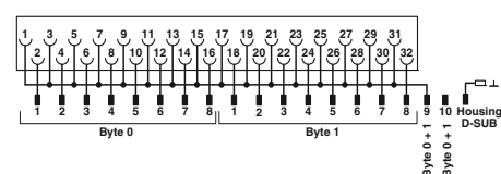
FLKM-PA-2D15/HW/DI/C300 connection scheme
