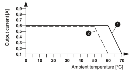
Derating curve ELR H3-IES-SC-230AC/500AC-0,6 100% operating time
