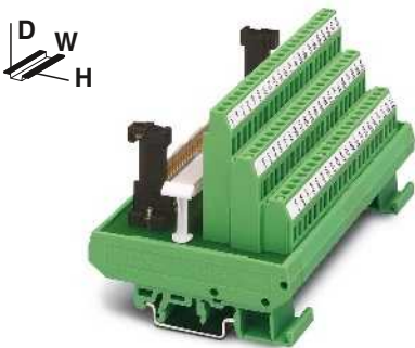
Design C, 64-position, a, c assembled
