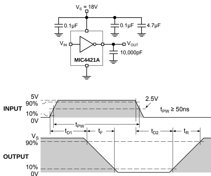
Figure 1. Inverting Driver Switching Time
