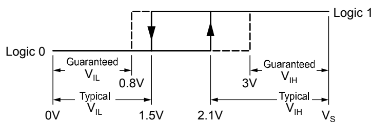
Figure 3. Input Hysteresis
