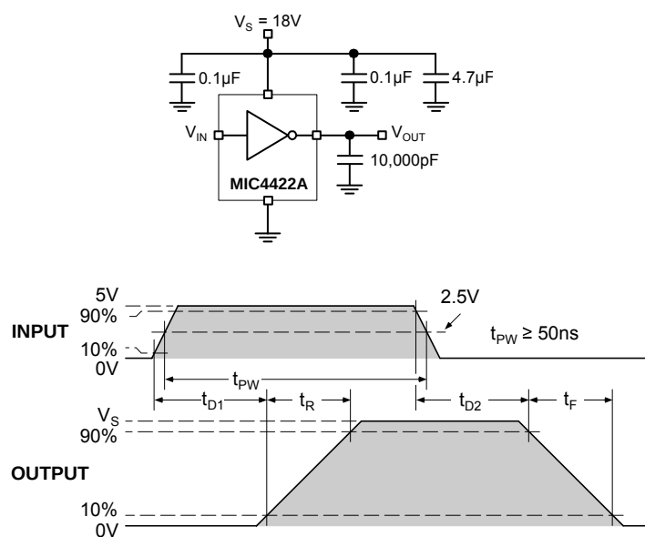
Figure 2. Non-Inverting Driver Switching Time
