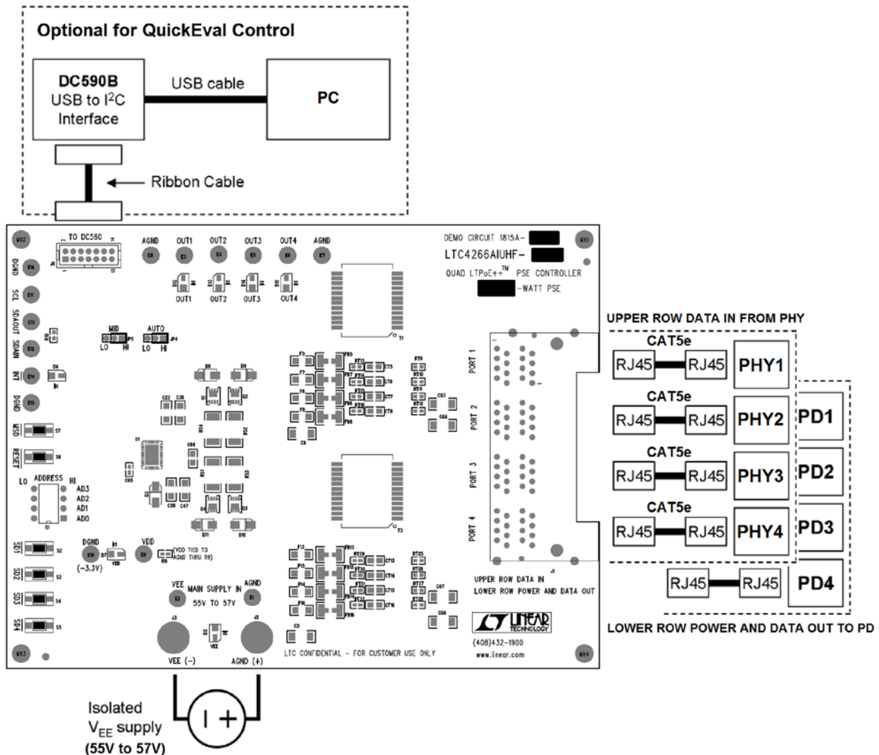
Figure 1. DC1815A Setup
