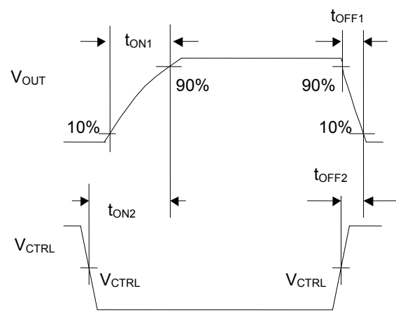
Figure 2. Timing Diagram
