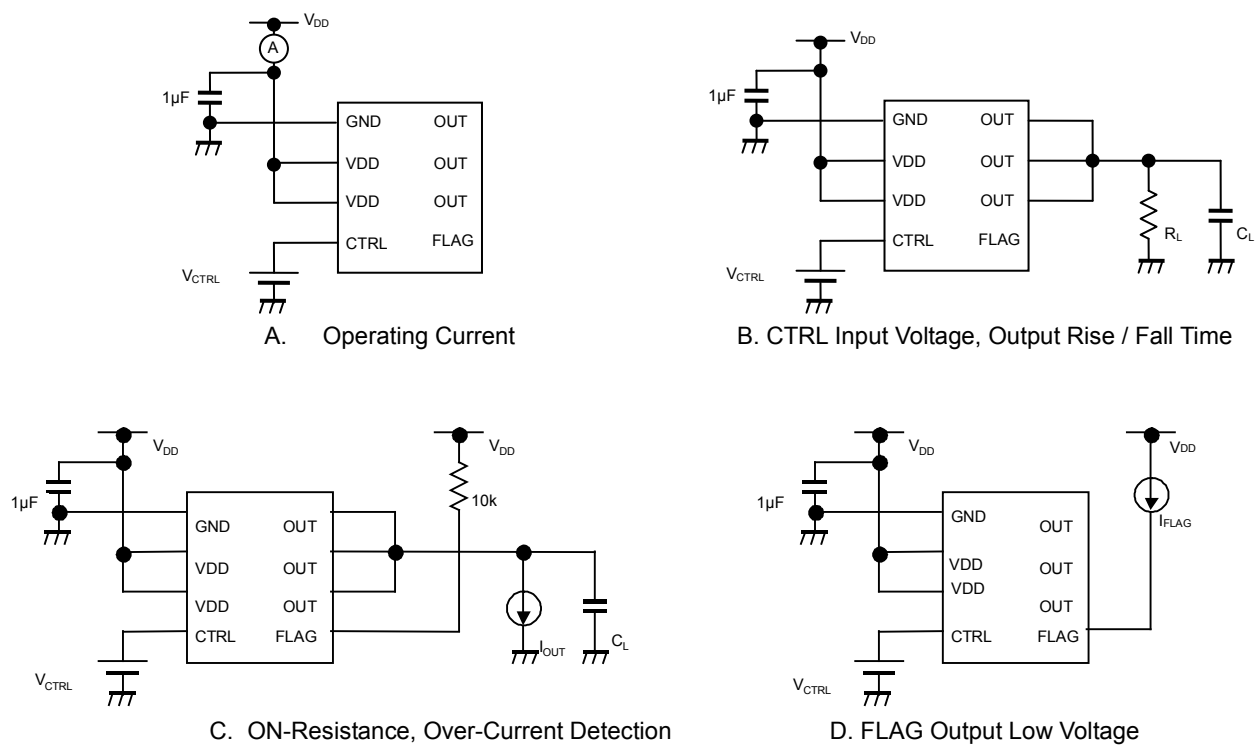
Figure 1. Measurement Circuit
