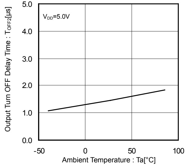
Figure 24. Output Turn OFF Delay Time vs Ambient Temperature
