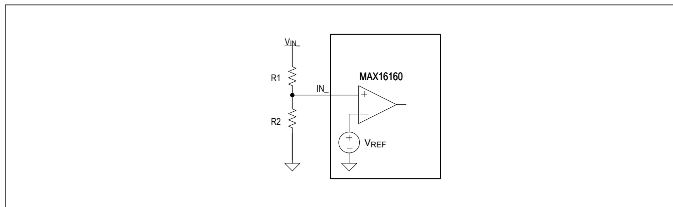
Figure 4. Adjustable Input Circuit
