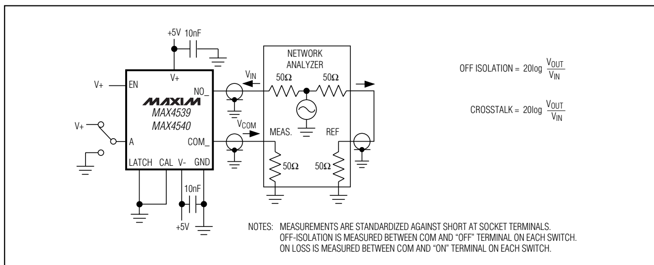
Figure 5. Off-Isolation/Crosstalk
