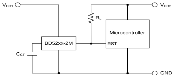
Figure 1. Open Drain Output Type BD52xx-2M Series
