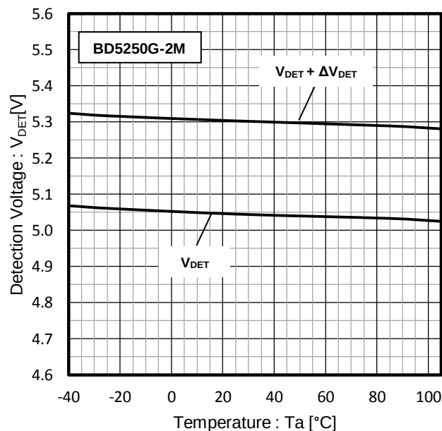
Figure 16. Detection Voltage and Release Voltage
