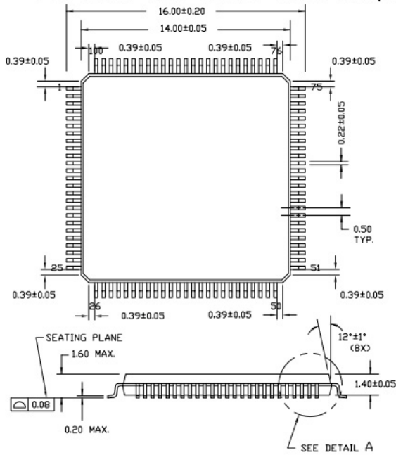
Figure 12. 100-pin TQFP (14 × 14 × 1.4 mm) A100SA
