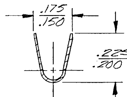
SECT. B-B
