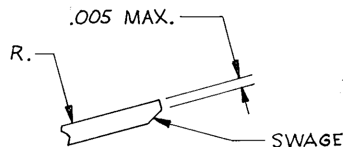
DETAIL C
