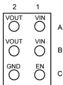
6-Ball 0.84mm × 1.32mm CSP (CS) Ball View
