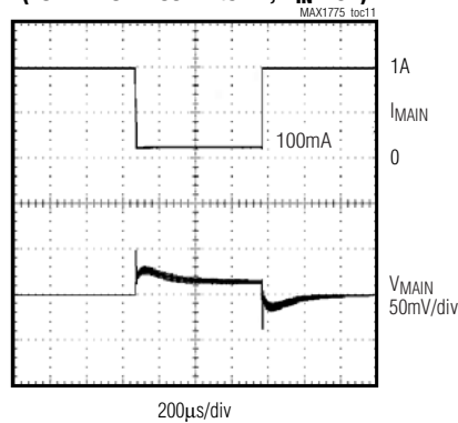
MAIN LOAD TRANSIENT (LOAD FROM 100mA TO 1A, V_{\text{IN}} = 5\text{V} )
