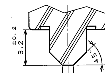
SECT. D-D (SCALE 5:1)
