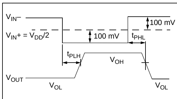
FIGURE 1-2: Propagation Delay Timing Diagram.
