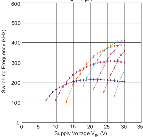
ZXLD1360 Switching Frequency L = 47µH
