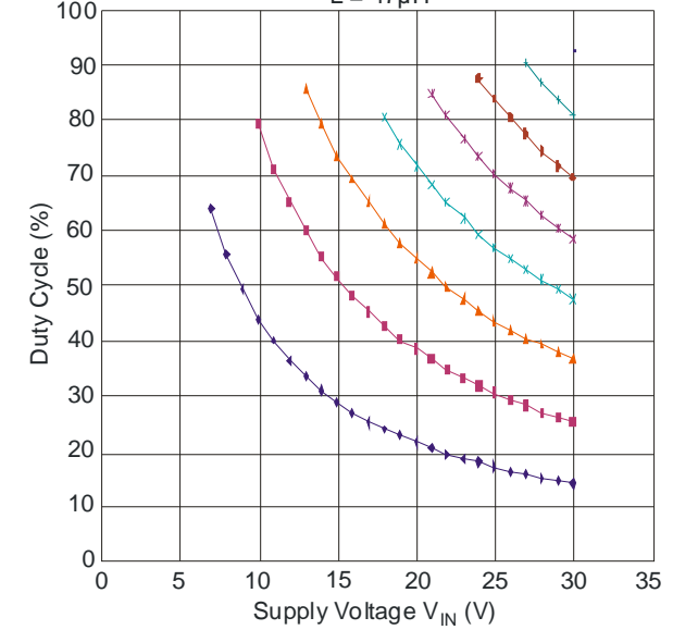
ZXLD1360 Duty Cycle L = 47µH
