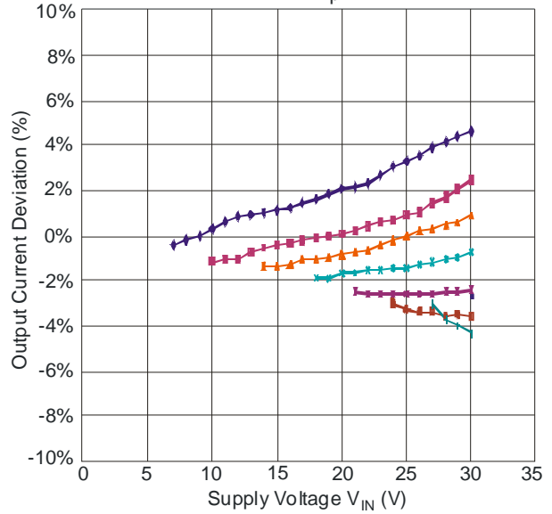
ZXLD1360 Output Current L = 47µH
