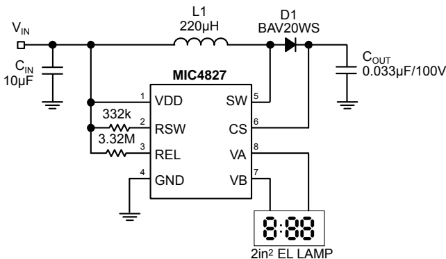
High Voltage EL Driver
