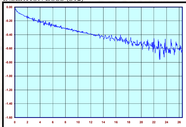
PN: CCSMA26.5-MM-086-5 INSERTION LOSS (S12)
