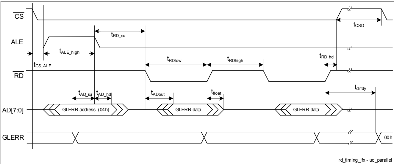
Figure 4 Timing by Parallel Read Access (e.g. GLERR Register)
