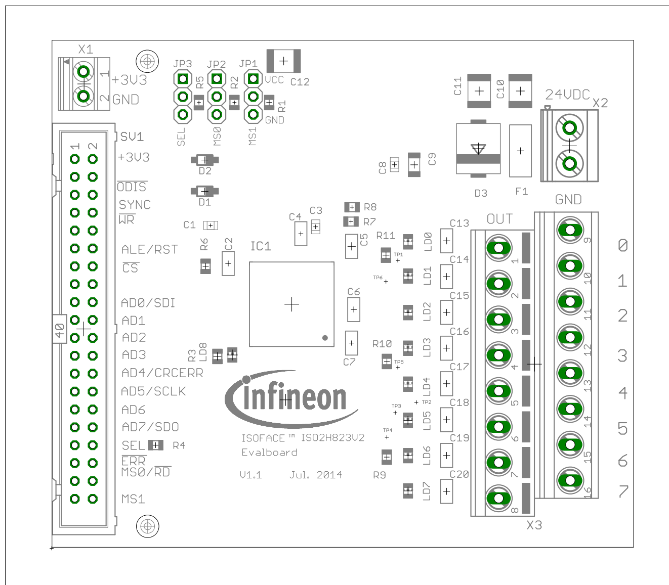
Figure 19 Component Placement
