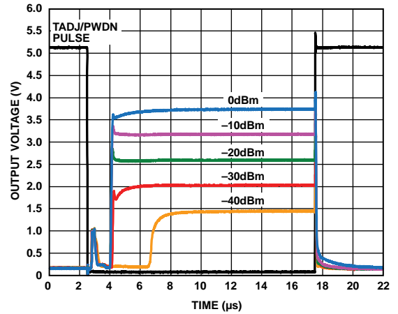
Figure 31. Output Response Using Power-Down Mode for Various RF Input Levels, Carrier Frequency = 2.14 GHz, C_{RMS} = 1 \text{ nF}
