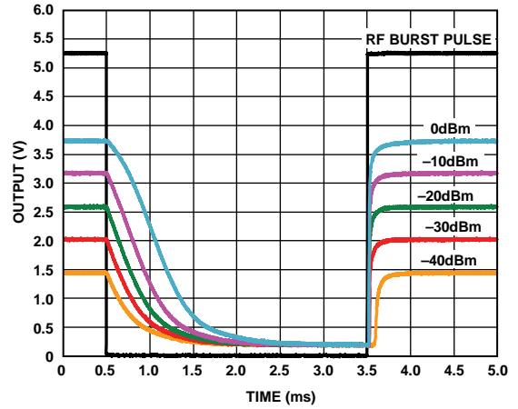
Figure 30. Output Response to RF Burst Input, Carrier Frequency = 2.14 GHz, C_{RMS} = 0.1 \mu\text{F}
