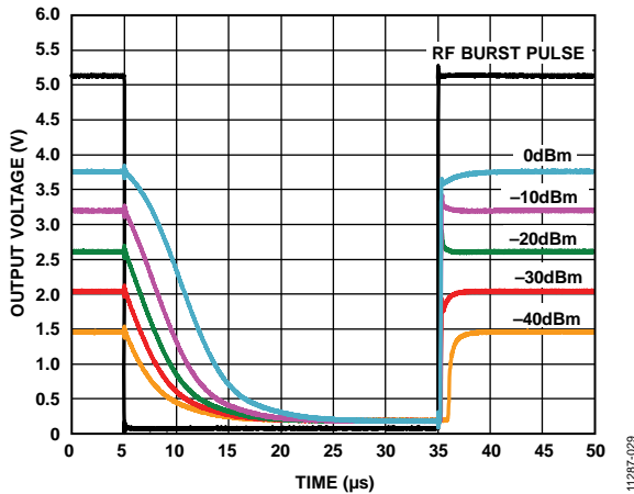
Figure 29. Output Response to RF Burst Input, Carrier Frequency = 2.14 GHz, C_{RMS} = 1 \text{ nF}
