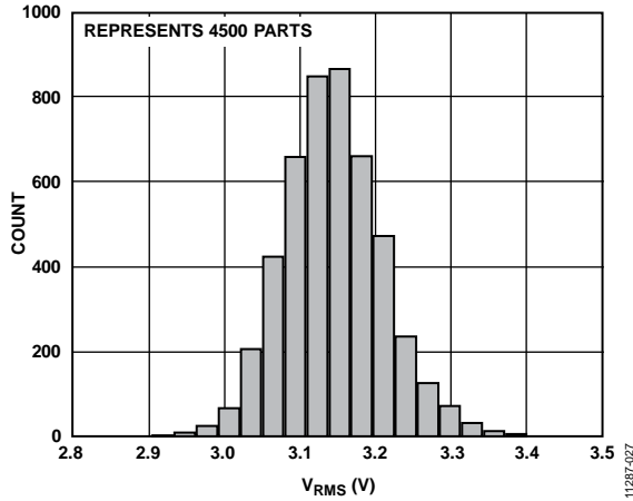
Figure 27. Distribution of V_{RMS} , P_{IN} = -10 \text{ dBm} , 900 MHz
