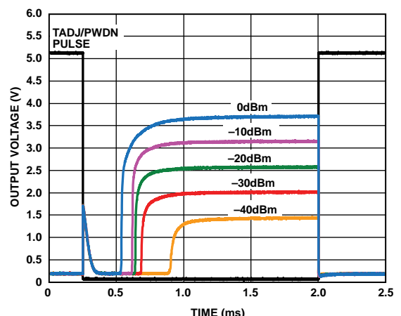
Figure 32. Output Response Using Power-Down Mode for Various RF Input Levels, Carrier Frequency = 2.14 GHz, C_{RMS} = 0.1 \mu\text{F}
