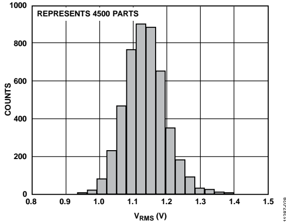
Figure 28. Distribution of V_{RMS} , P_{IN} = -45 \text{ dBm} , 900 MHz
