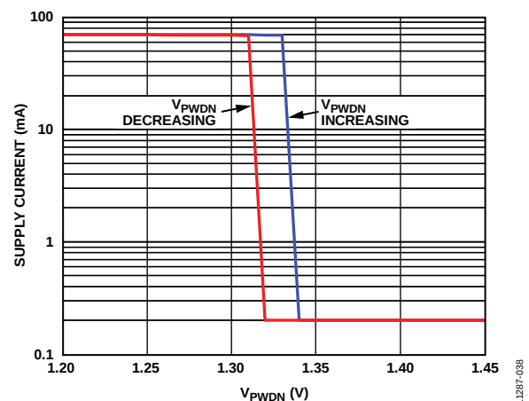
Figure 38. Supply Current vs. V_{PWN}
