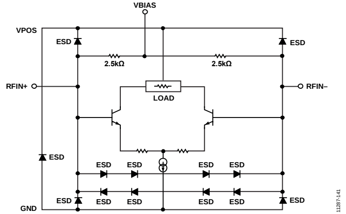
Figure 42. RF Inputs
