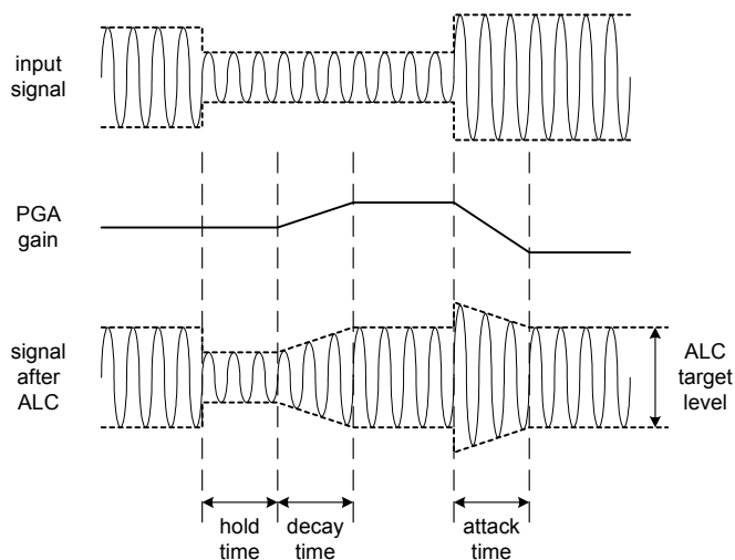
Figure 10 ALC Operation
