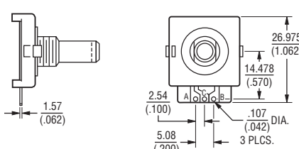
PCB MOUNTING DIMENSIONS
