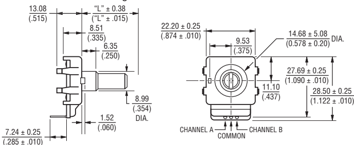
Shaft Style B
