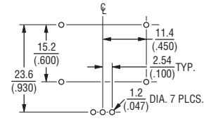
PCB MOUNTING DIMENSIONS (Housing Styles B and E)
