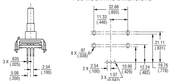
Shaft Style R
