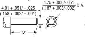
Shaft Style J
