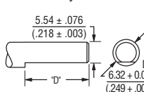
Shaft Style C
