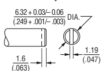
Shaft Style B
