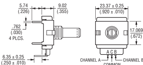
SNAP-IN MOUNT - Housing G
