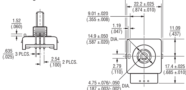
BUSHING MOUNTED - HOUSING H
