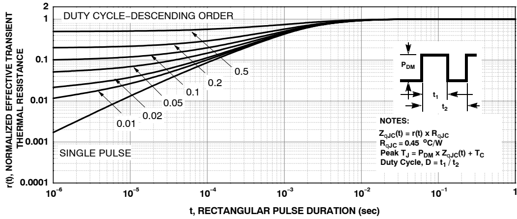
Figure 8. Junction-to-Case Transient Thermal Response Curve
