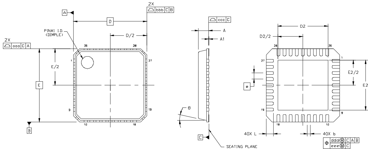
Figure 9. 36-Pin Quad Flat No-lead (QFN)
