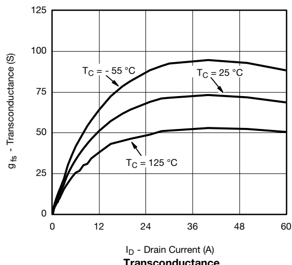
Transconductance
