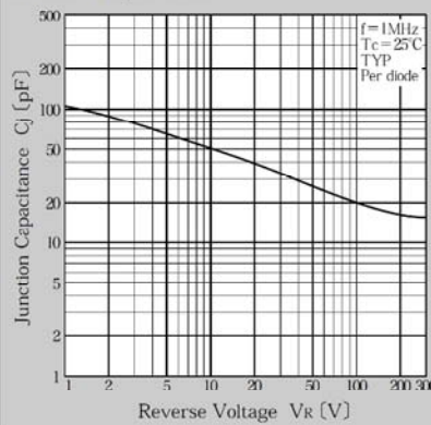
Junction Capacitance
