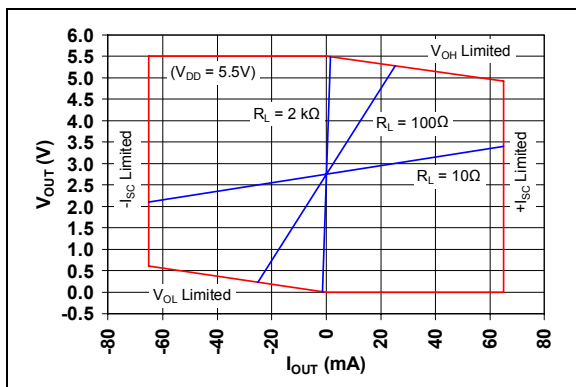
FIGURE 4-6: Output Current.
