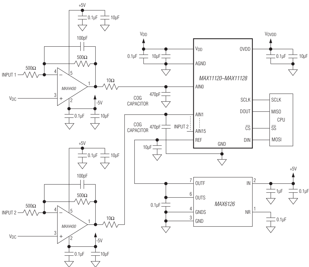
Figure 13. Typical Application Circuit
