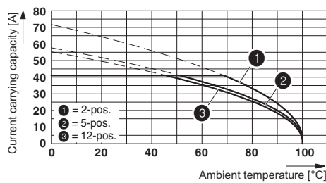
Derating curve for: IPC 5/...-ST-7.62 with IPC 5/...-G-7.62 Conductor cross section = 10 mm 2
